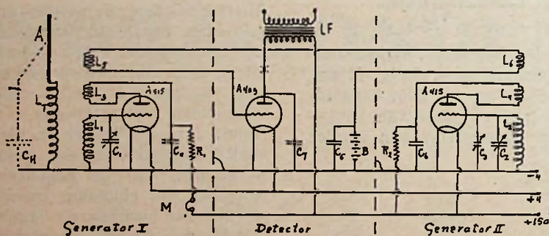
Principe-schema Theremin-apparaat
